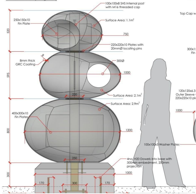
01 - Front Elevation (Through View)
